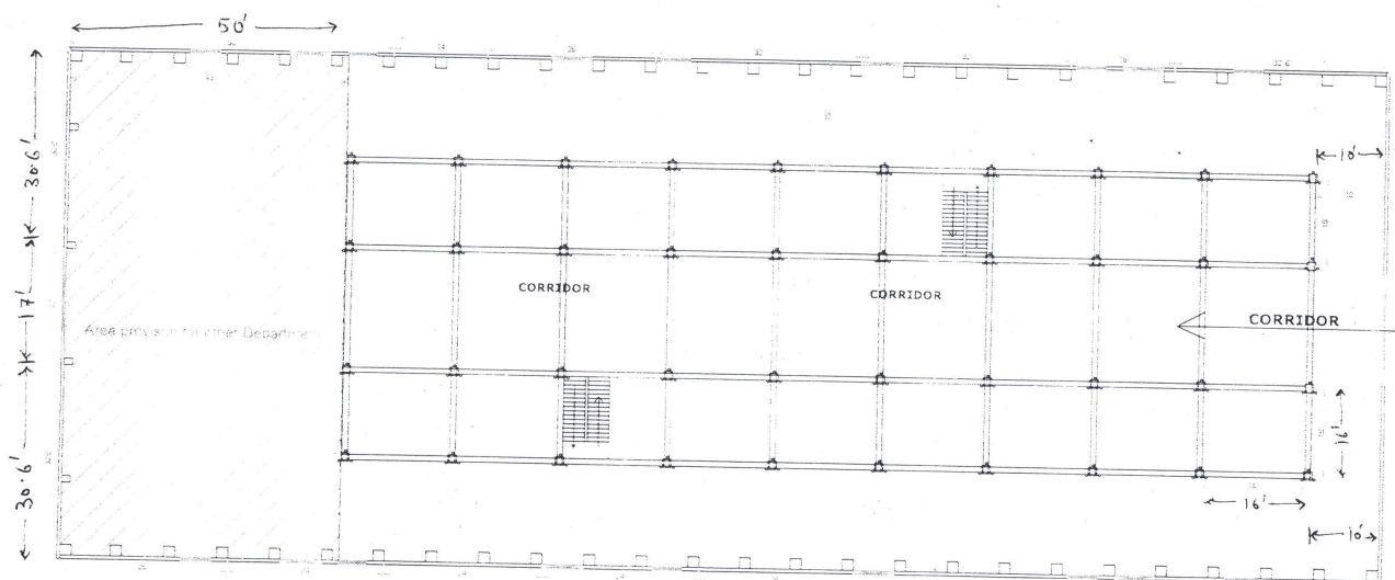
PROPOSED LAYOUT FOR STEEL COULOMB AND BEAM FOR WOODEN FLOORING IN MECHANICAL WORKSHOP.
